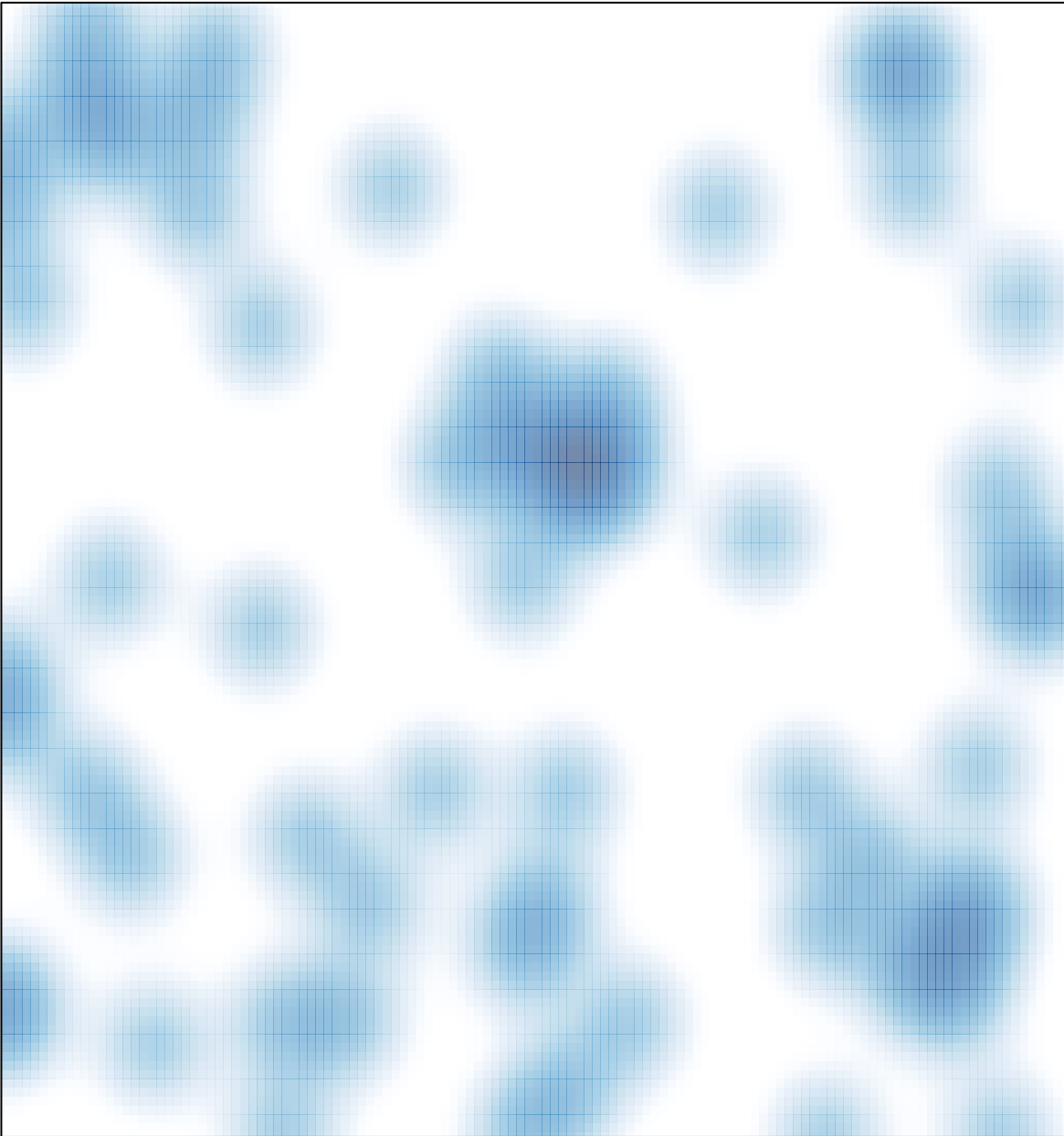
# features = 64 , max = 2
